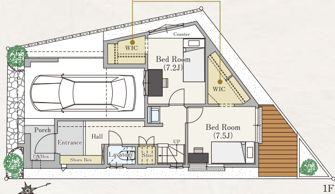
1F
